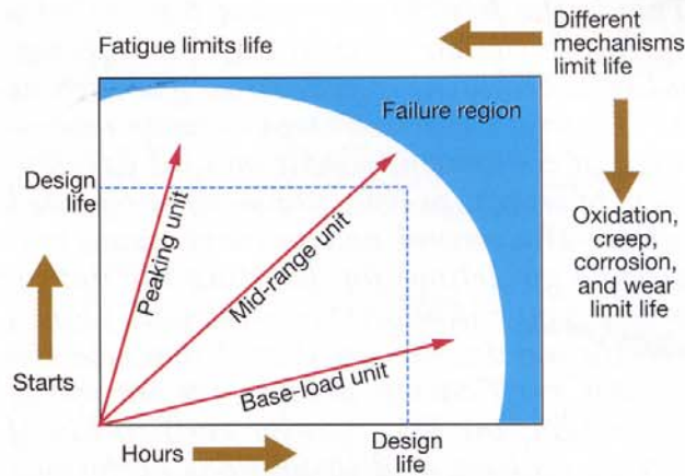
1-5. Assessment of equipment condition should determine the need for refurbishment, not theoretical assumptions based on starts and operating hours as shown
