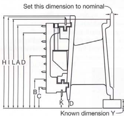
2-6. Dimensional checks conducted by the repair shop are necessary to determine such things as downstream deflection of nozzle or vane segments
